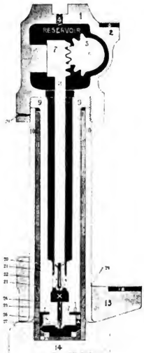
Fig. 4580. Hydraulic Claw Jack. A. L. Henderer's Sons.
